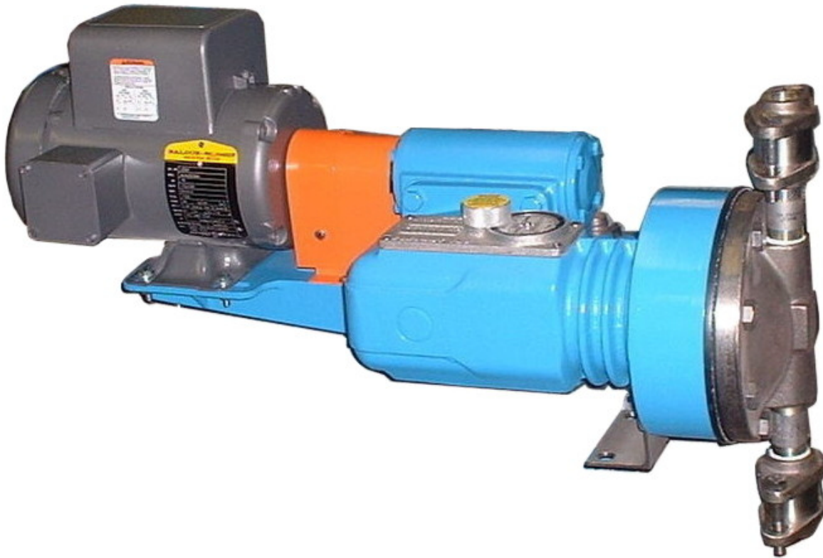
MH Series Simplex pump. Shown with optional variable speed motor.
